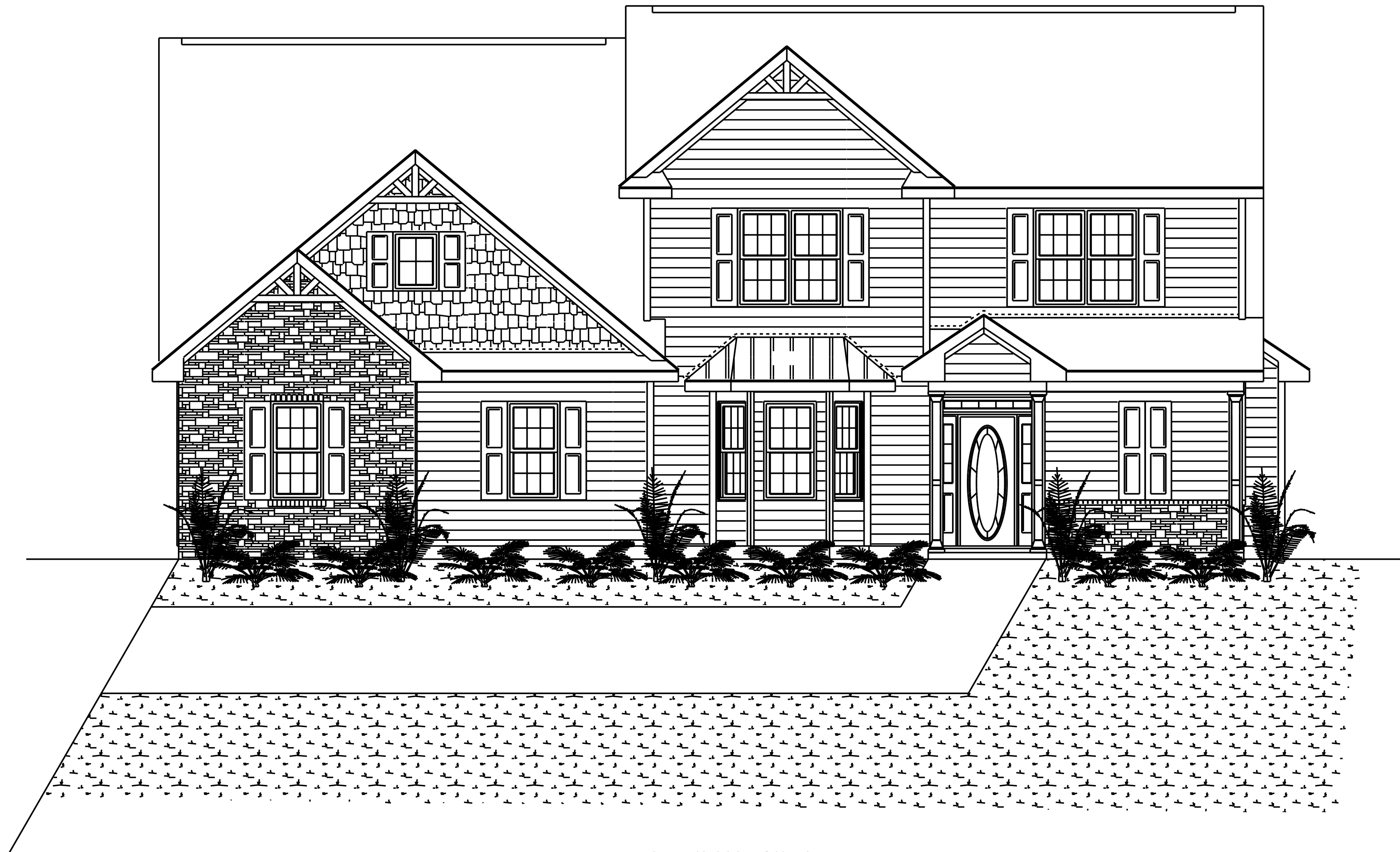
FRONT ELEVATION
